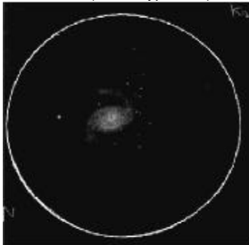
M33 (Triangulum)
