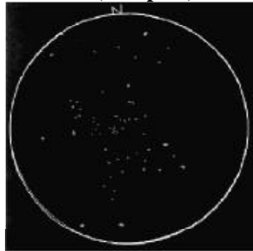
M7 (Scorpius)
